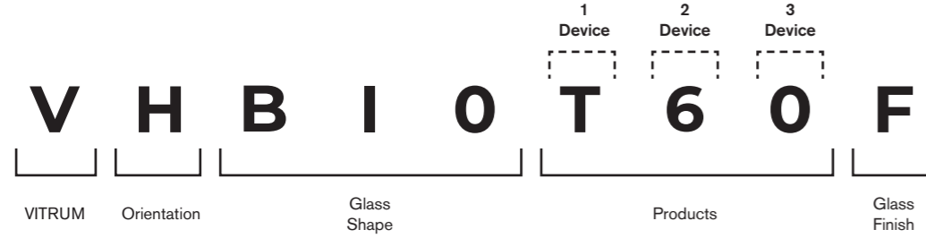
Combined Faceplate - Example 1
